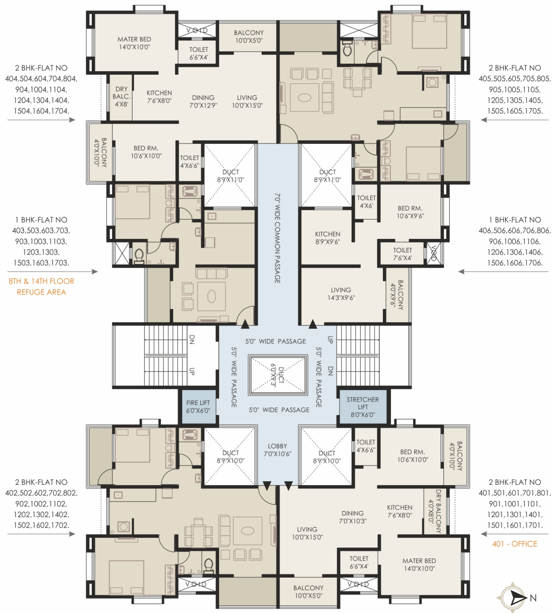
TYPICAL 4TH, 5TH, 6TH, 7TH, 8TH, 9TH, 10TH, 11TH, 12TH, 13TH, 14TH, 15TH, 16TH & 17TH FLOOR PLAN
